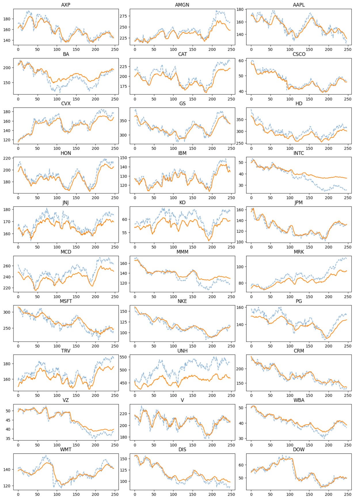
Fig. 6. LSTM2D results.
